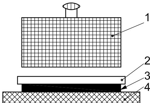
c) Adhesive failure between tile and pull-head plate — BF
