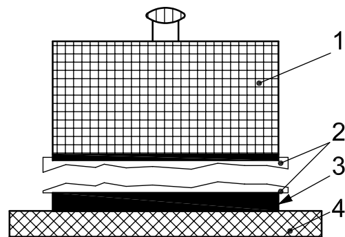
f) Cohesive failure within the tile — CF-T
