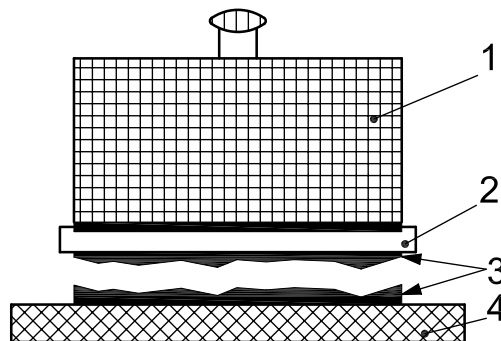
d) Cohesive failure within the adhesive — CF-A
