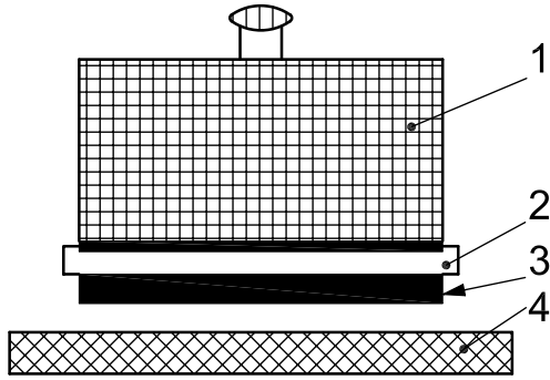
a) Adhesive failure between adhesive and substrate — AF-S
