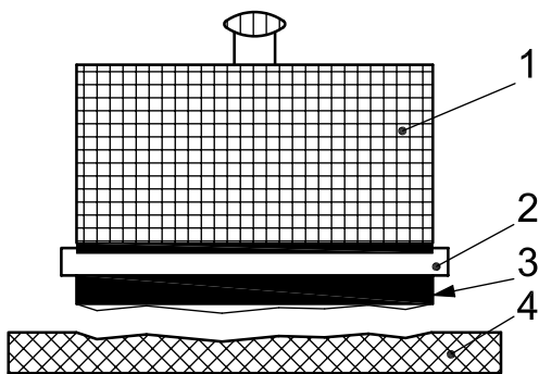
e) Cohesive failure within the substrate — CF-S
