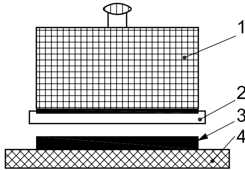
b) Adhesive failure between tile and adhesive — AF-T
